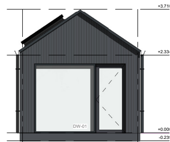
FACADE ON AXIS B-A M 1 : 50
